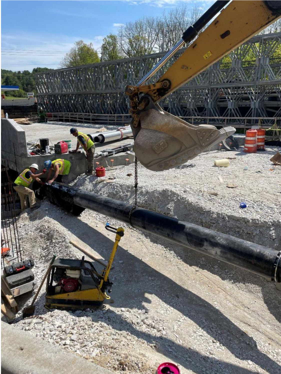
New waterline being installed near Abutment #2
